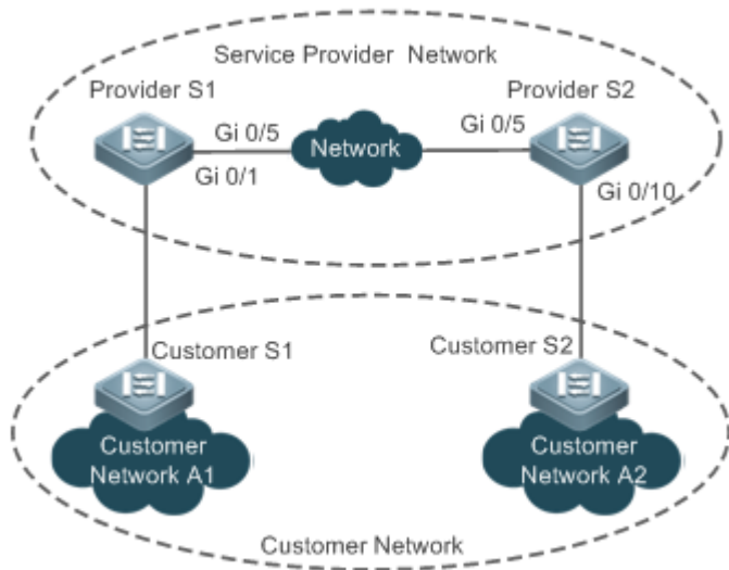
Figure 9-2 BPDU Tunnel Topology
