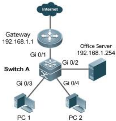
Figure 20-1 Typical Topology of Gateway-targeted ARP Spoofing Prevention
