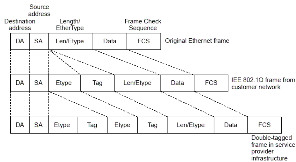
Figure 12-1 Outer Tag Encapsulation
