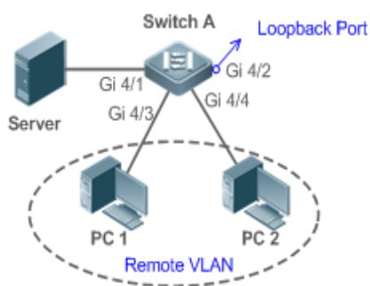
Figure 5-3 Application Topology of One-to-Many RSPAN
