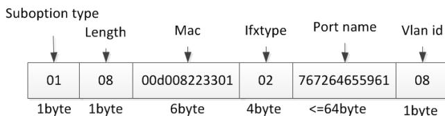
Figure 4-9 Option82-remote-id
