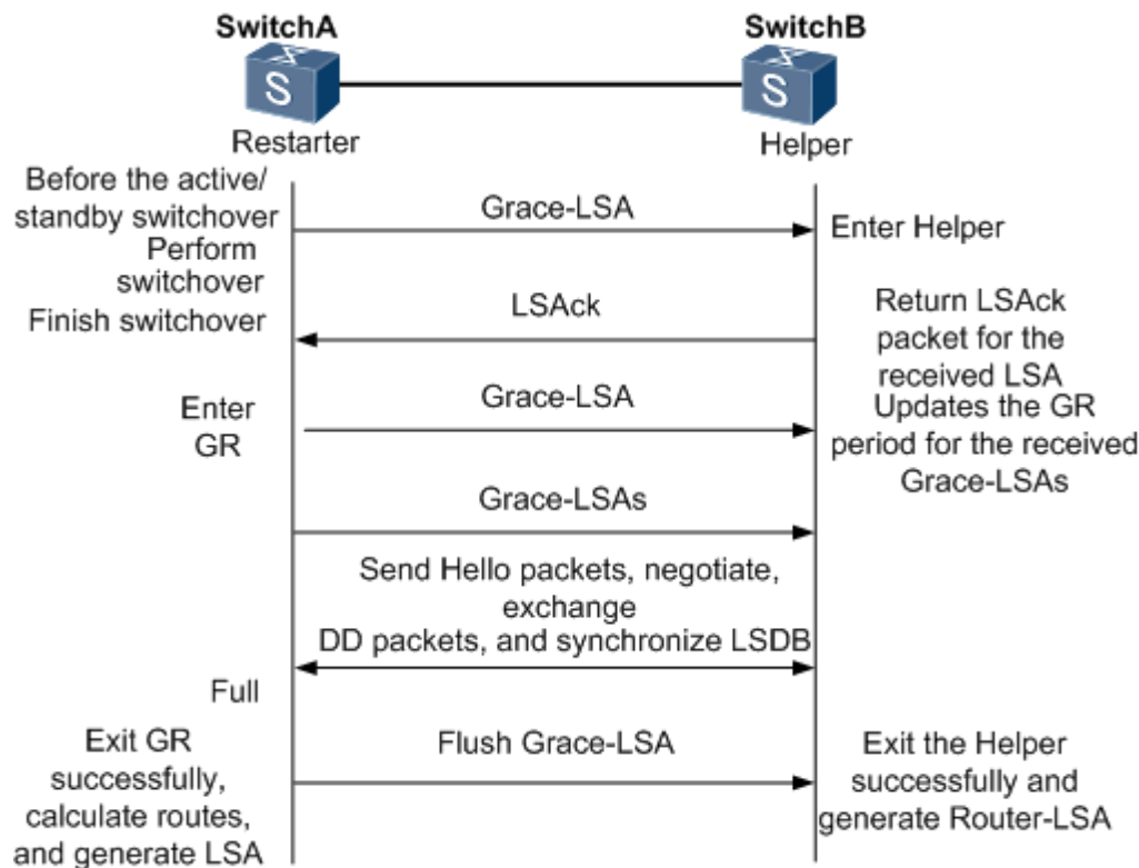
Figure 3-6 Normal OSPF GR Process
