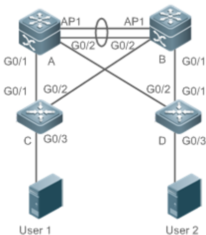
Figure 9-1 MSTP+VRRP Dual-Core Topology
