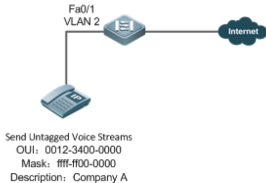
Figure 8-2 Networking When the Voice VLAN Works in Manual Mode
