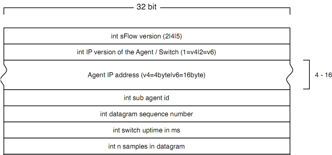
Figure 7-3 sFlow Header
