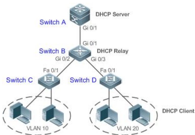
Figure 4-3 DHCP Relay
