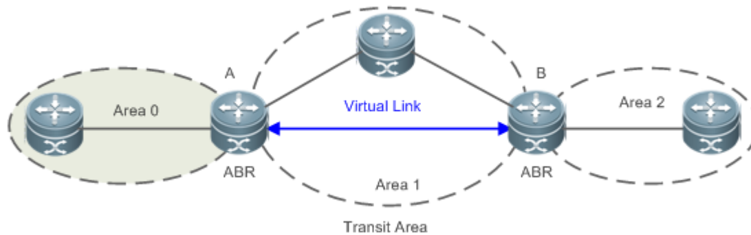
Figure 3-4 Failure to Directly Connect a Normal Area to the Backbone Area on the Physical Network
