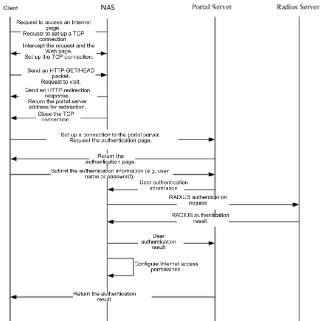
Figure 5-3 Flowchart of Nodexon Second-Generation Web Authentication
