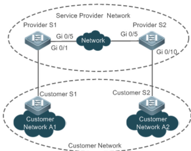
Figure 10-2 GVRP PDUs Tunnel Application Topology
