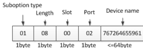
Figure 4-9 Option82-remote-id
