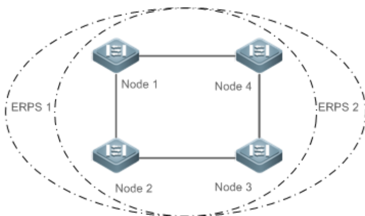
Figure 13-4 Single-Ring Load Balancing
